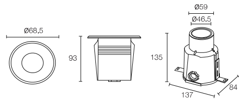
Mounting sleeve
